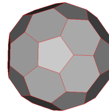
C_{60}
