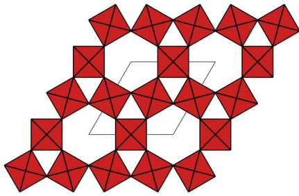
WO 3 (hexagonal)
