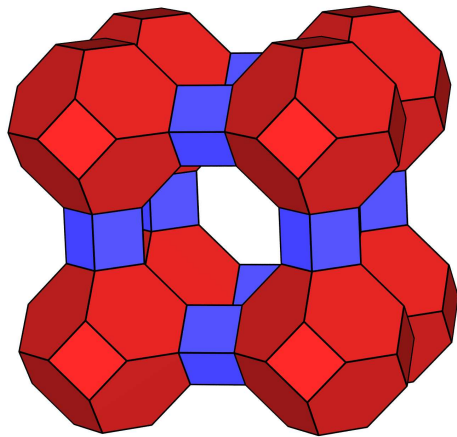
Zeolith A
